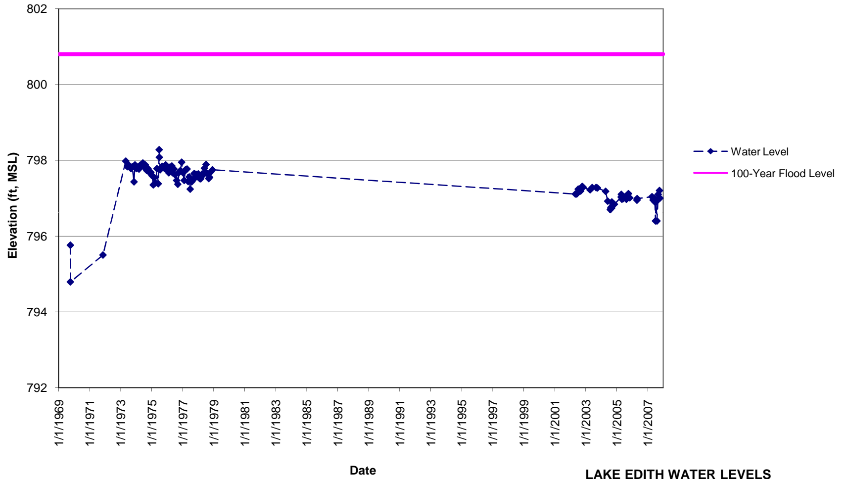
LAKE EDITH WATER LEVELS Valley Branch Watershed District
